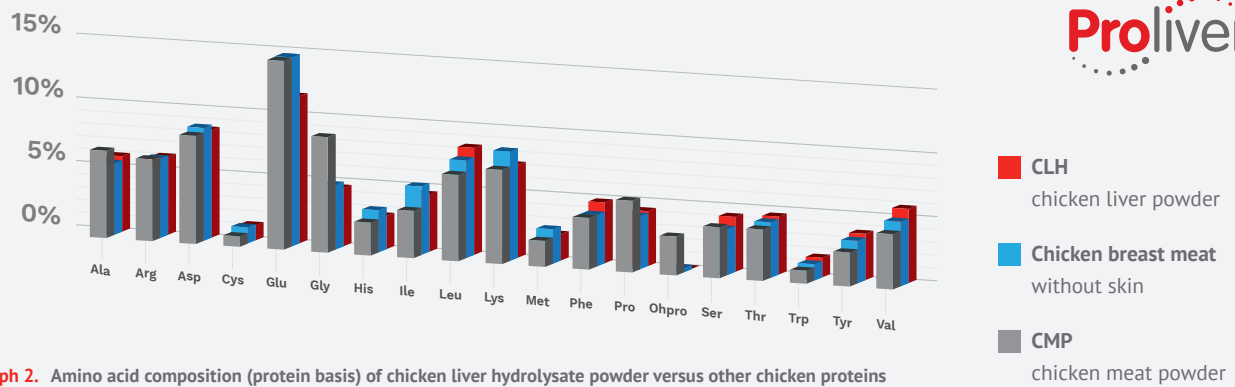
graph 2. Amino acid composition (protein basis) of chicken liver hydrolysate powder versus other chicken proteins
