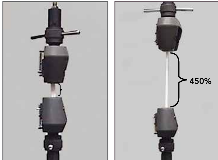
DEK-650 Flexible Membrane achieves 450% elongation as performed by ASTM D638.
