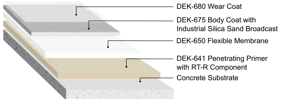
DEK-650 Flexible Membrane achieves 450% elongation as performed by ASTM D638.
